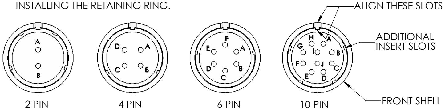
FIG 6 VIEW A-A
